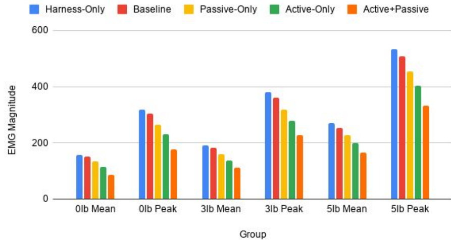
a) EMG Data of the Flexion Motion
