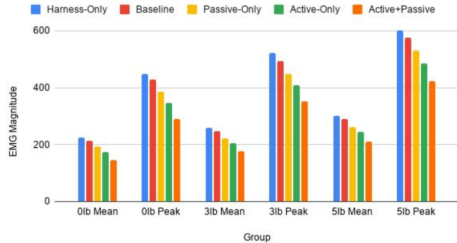
b) EMG Data of the Abduction Motion
